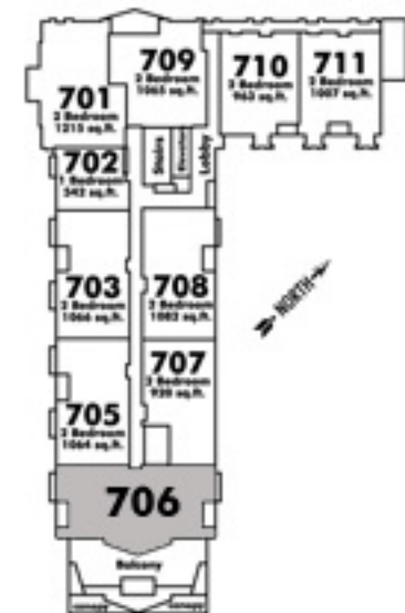
7th Floor
